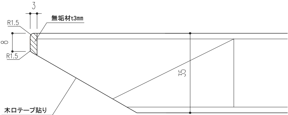
Detail S=1:1
